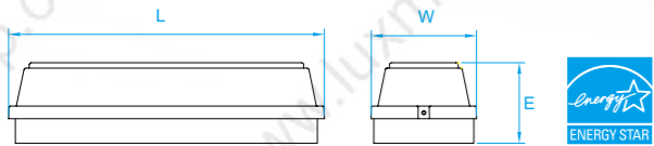
Model No. LO014 Dimension 13-3/8"L x 4-1/2"W x 3-1/2"E Lamp (2) medium or GU24 base 16W integral LED 1400 lumens
