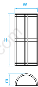
Model No. LW108 Dimension 7"W x 16"H x 3-3/4"E Lamp (2) medium or GU24 base 16W integral LED 1050 lumens
