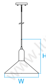
Model No. LP247 Dimension 13-3/4"W x 10-3/4"H Lamp (1) medium or GU24 base
