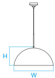
Model No. LP268 Dimension 23-1/2"W x 26-5/8"H Lamp 37W integral LED 3000 lumens
