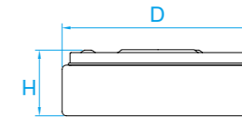
Model No. LC273 Dimension 11"D x 4-1/2"H Lamp (1) medium or GU24 base 18W integral LED 1340 lumens
