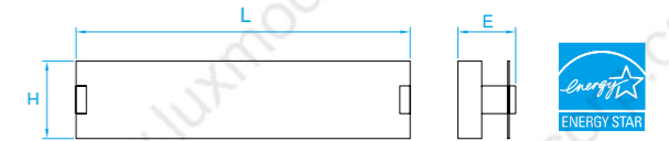
Model No. LV276 Dimension 19"L x 4-3/4"H x 3-1/2"E Lamp 24W integral LED 1700 lumens
