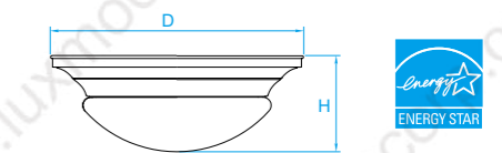
Model No. LC002 Dimension 14-3/8"D x 5-1/2"H Lamp (2) medium or GU24 base 18W integral LED 1300 lumens
