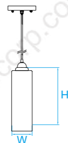
Model No. LP142 Dimension 4"W x 12"H Lamp (1) medium or GU24 base
