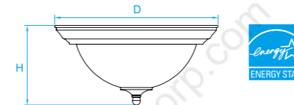
Model No. LC001 Dimension 13-3/8"D x 6-1/2"H Lamp (1) medium or GU24 base 18W integral LED 1300 lumens
