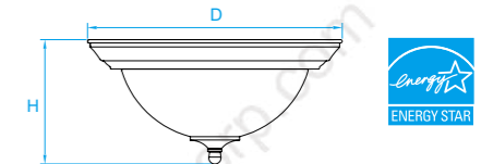
Model No. LC227 Dimension 15-1/4"D x 6-3/4"H Lamp (2) medium or GU24 base 25W integral LED 2160 lumens
