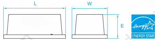
Model No. LO013 Dimension 10-1/2"L x 6"W x 4-1/4"E Lamp (1) medium or GU24 base 14W integral LED 1300 lumens
