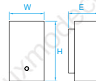
Model No. LV138 Dimension 4-3/4"W x 7-1/2"H x 4"E Lamp (1) medium or GU24 base
