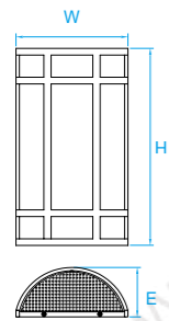
Model No. LW043 Dimension 8-7/8"W x 14"H x 3-1/2"E Lamp (2) medium or GU24 base 16W integral LED 1100 lumens
