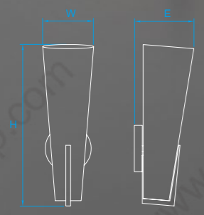
Model No. LW193 Dimension 5"W x 15-1/2"H x 5-3/4"E Lamp 15W integral LED 900 lumens
