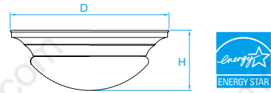
Model No. LC070 Dimension 12-1/8"D x 4-5/8"H Lamp (1) medium or GU24 base 18W integral LED 1300 lumens
