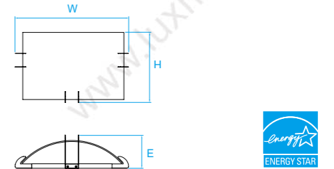
Model No. LW013 Dimension 16-1/2"W x 9-4/5"H x 4-3/4"E Lamp (2) medium or GU24 base 14W integral LED 1150 lumens
